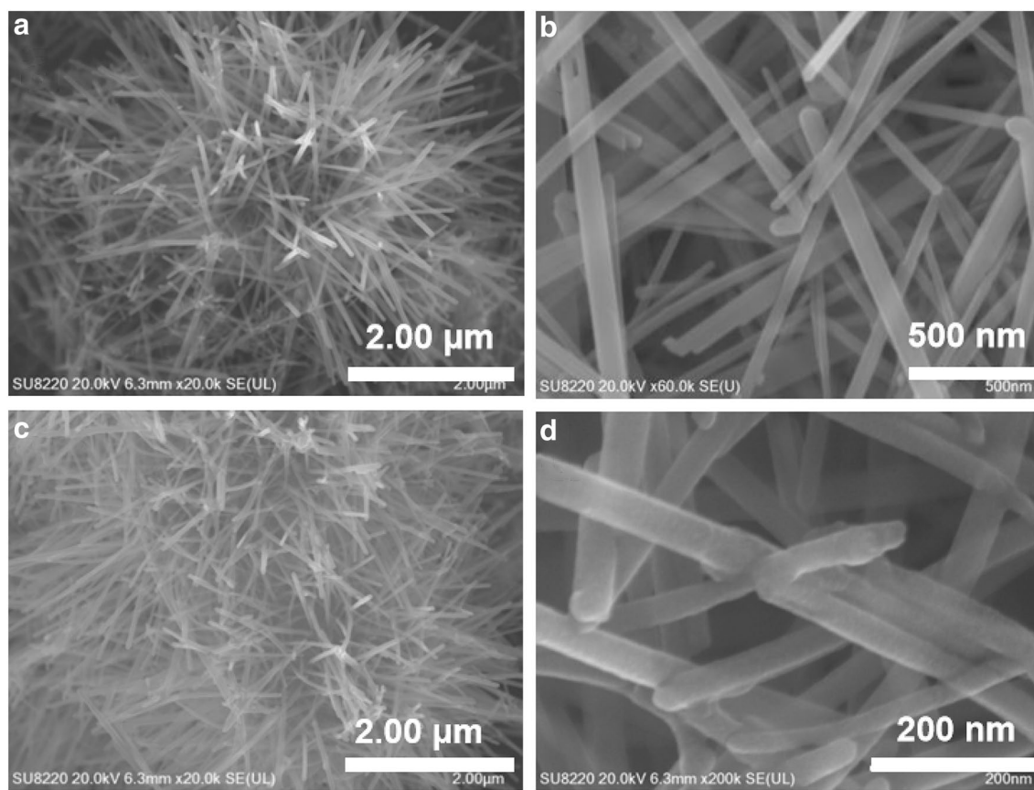
Fig. 1 a, b SEM images of the pure MnO 2 nanorods; c, d SEM images of the MnO 2 @C composite nanorods
