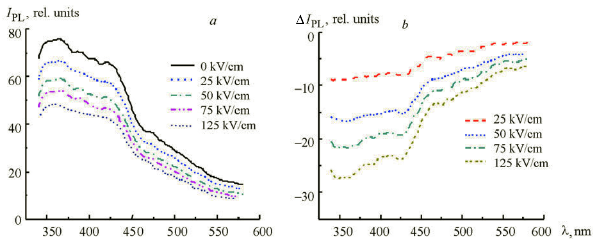
Fig. 5. Photoluminescence excitation (a) and differential excitation (b) spectra of CdSe nanorods with average particle length/diameter 20:5 nm (matrix layer thickness \Delta h_M \sim 40 \mu\text{m} ) in external electric fields of 0 to 125 kV/cm; \lambda_{\text{det}} = 630 \text{ nm} .
