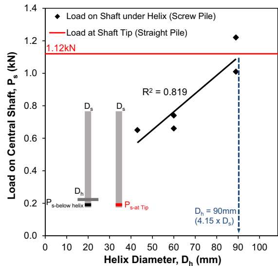
Fig. 6 Load distribution under the helix with increasing helix diameter a comparison of load on central shaft under helix with straight pile tip load
