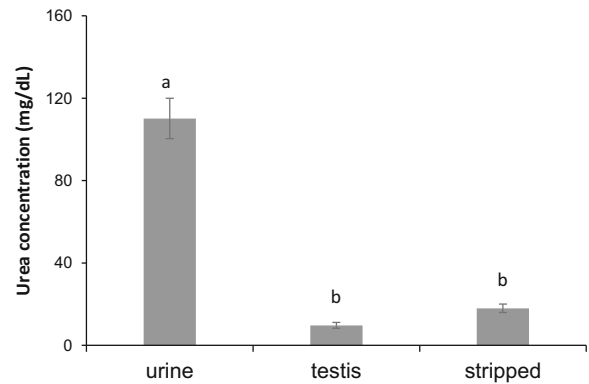
Fig. 2 Differences in urea concentrations (mg/dL) in spotted wolffish pure urine samples and seminal plasma obtained from testes sperm and by stripping. Different letters stand for significant differences between group of samples as detected with a one-way ANOVA ( p < 0.05 ). Values represent the mean \pm SEM
