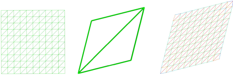
Fig. 4 Periodic stable 2D structure under in-plane loading. Solution of corrector problem \chi^{12} and approximation of the solution for \mathcal{U}(x_1, x_2) = x_2 \mathbf{e}_1 + x_1 \mathbf{e}_2
