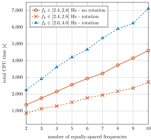
Fig. 13 Total CPU times of MSSS-IDR(4) for N_\omega > 1 frequencies equally-spaced within a fixed range. Additional scaling (dashed lines) following [7] improves convergence, and allows for larger frequency ranges
