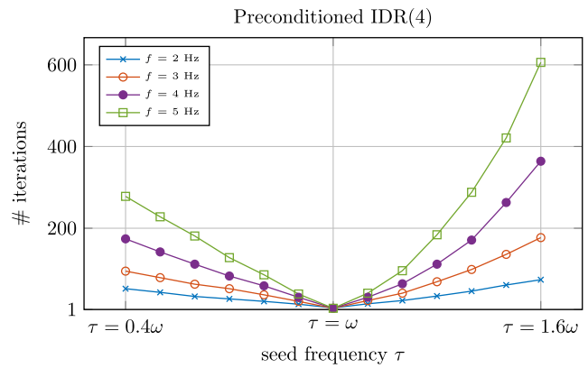
Fig. 11 Number of iterations of preconditioned IDR( s ) when \tau \neq \omega in (19). We perform the experiment for different frequencies, and keep a constant grid size h = 5m and residual tolerance \text{tol} = 10\text{e-}8
