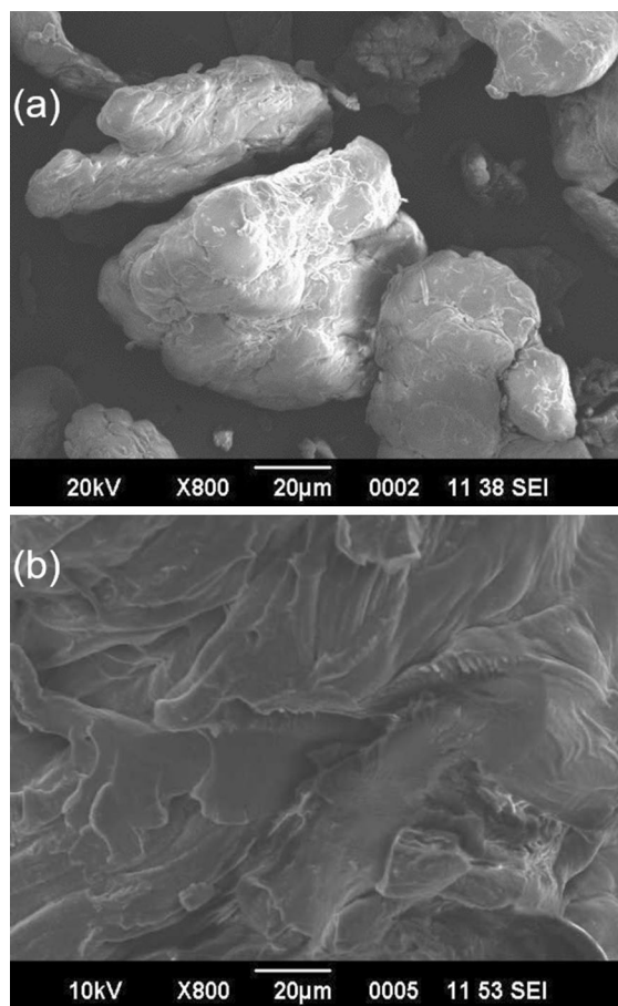
Fig. 6 Scanning electron micrographs of a HPMC and b HPMC-g-PAM 10
