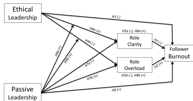
Fig. 1 Theoretical model
