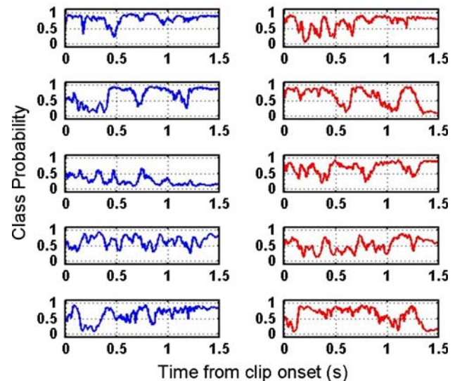
Fig. 1 Probability of the model B1 of predicting that class was happy when the actual clip evolves to happy (left plot) or to predict that clip was angry when the actual clip evolves towards angry (right). Probabilities are displayed as a function of time (seconds) from clip onset. One subject is depicted on each row. Probability values near to one indicate that the correct class was identified for the subject
