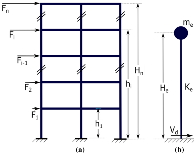
Fig. 1 The MDOF structure (a) and its SDOF representation in the original DDBD (Sullivan et al. 2012) method (b)
