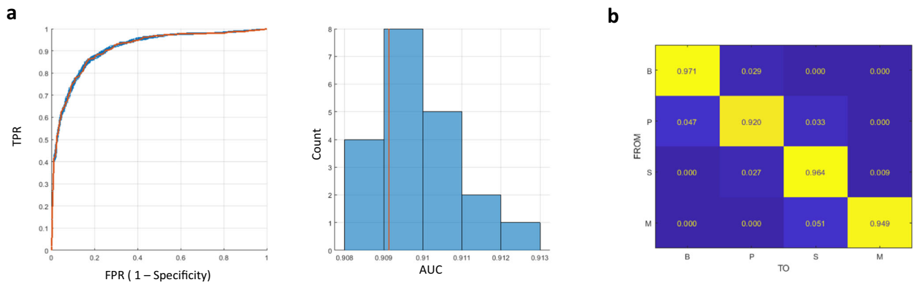
Fig. 5 Results of the system evaluation. a ROC curves and corresponding AUCS assessing impact of ROI boundary variation. b Assessment of class switching due to ROI boundary variation
