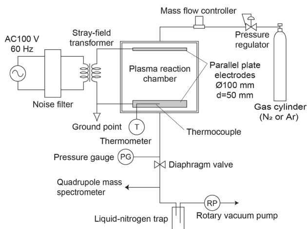
Fig. 1 Schematic diagram of glow-discharge plasma reactor
