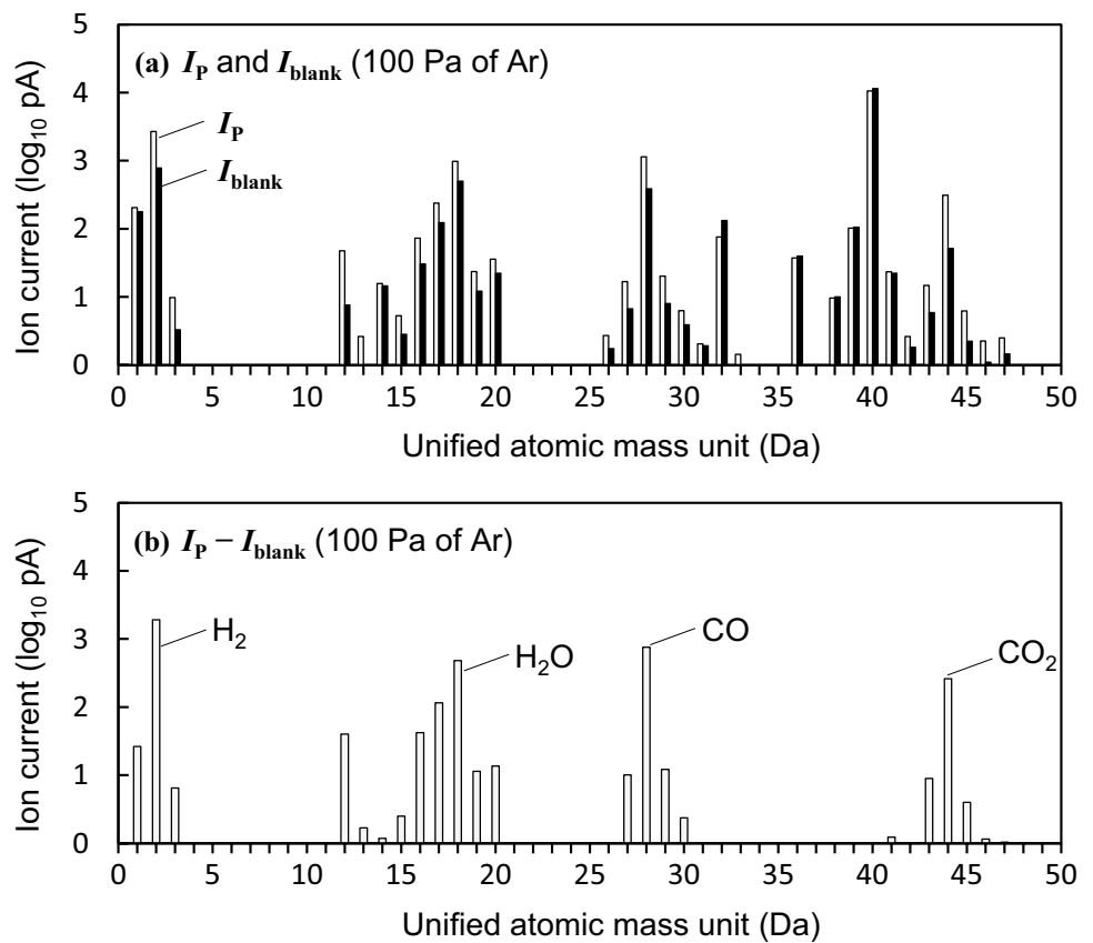
Fig. 8 Quadrupole mass spectrometry for gaseous products from filter papers treated by glow-discharge plasma with Ar at 100 Pa
