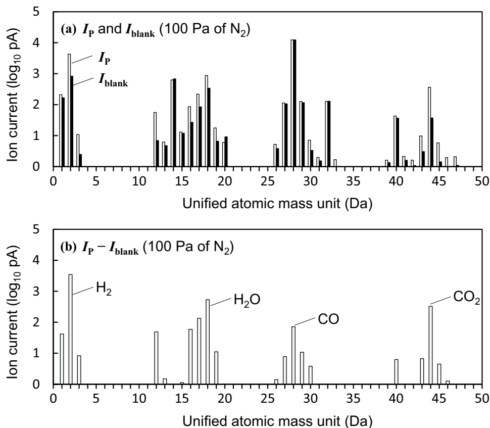
Fig. 7 Quadrupole mass spectrometry for gaseous products from filter papers treated by glow-discharge plasma with N_2 at 100 Pa/0.59 W
