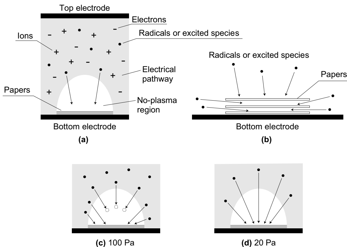
Fig. 6 Explanation for decomposition behavior of cellulose in glow-discharge plasma
