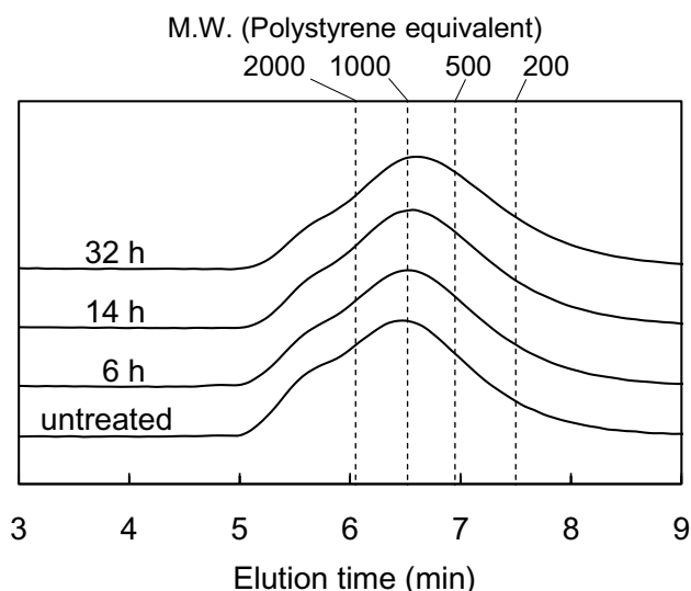
Fig. 5 Gel permeation chromatograms for THF-soluble portion of phenyl carbamate derivatives of filter paper treated in glow-discharge plasma with N 2 at 100 Pa/0.59 W
