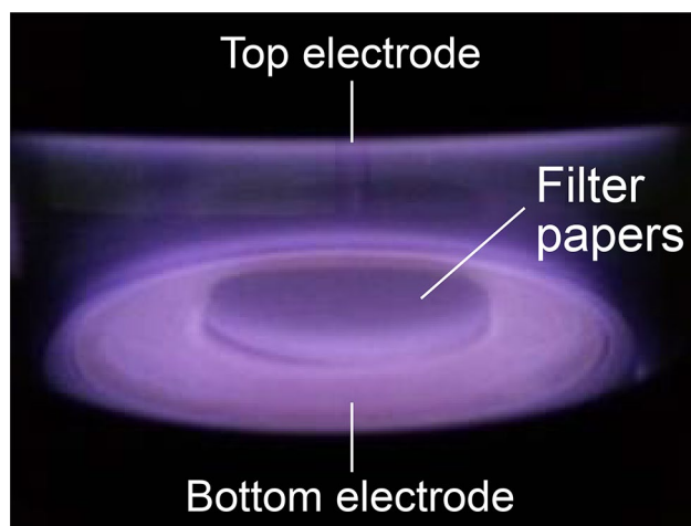
Fig. 2 Visual appearance of plasma treatment of filter papers under N_2 flow
