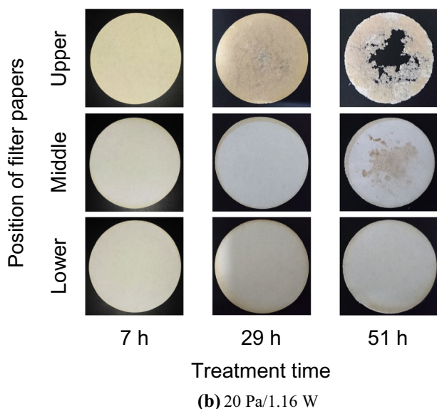
Fig. 4 Visual appearances of filter papers treated in glow-discharge plasma with N 2 at a 100 Pa/0.59 W and b 20 Pa/1.16 W
