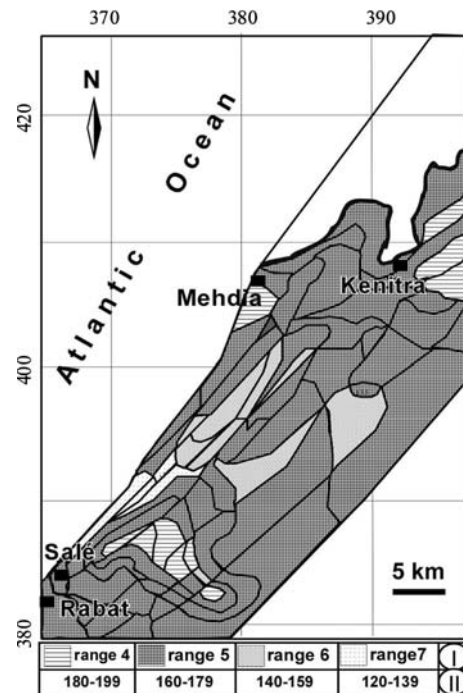
Fig. 7 Vulnerability map according to the DRASTIC method [I. Vulnerability ranges (Aller et al. 1987), II. intervals of Id values]
