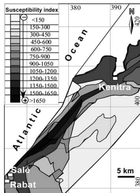
Fig. 8 Sensibility map according to the DRASTIC method and land use analysis
