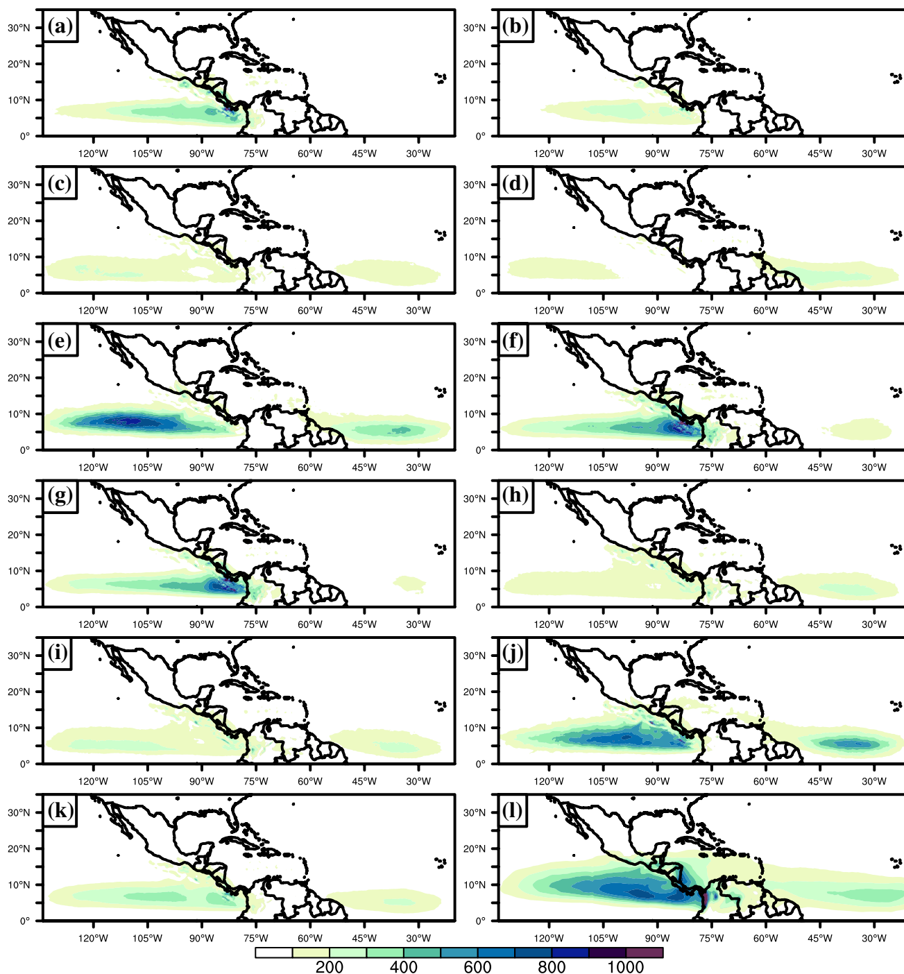
Fig. 12 Rainfall (mm) produced by easterly waves in ten members of the WRF ensemble: a ck6m, c cktm, e cn6y, g cnty, i ctty, b rk6m, d rktm, f rn6y, h rnty, j rtty, k ensemble mean and ERAI during the 1990–2000 period
