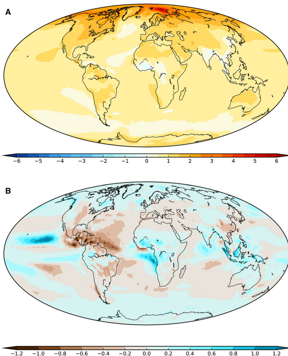
Fig. 1 a Ensemble mean temperature change for the period 1850–2005, unit °K. b The same for precipitation, unit mm/day. Change computed as average for last 10 years minus average for first 10 years
