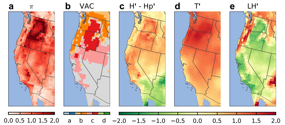
Fig. 7 Land atmosphere coupling metrics and anomalies for June 2015. a \tilde{\pi} metric, b VAC index, c sensible heat flux minus potential sensible heat flux anomaly H' - H_p' , d temperature anomaly T' and e latent heat flux anomaly LH'
