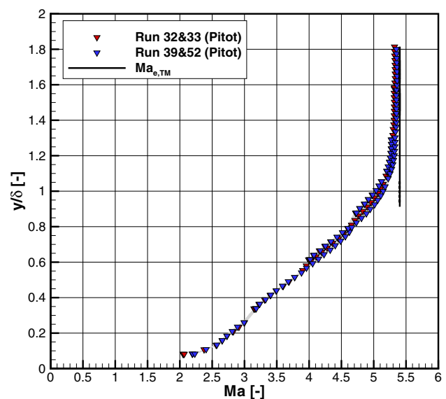
Fig. 3 Mach profiles of Pitot run 32&33 and 39&52
