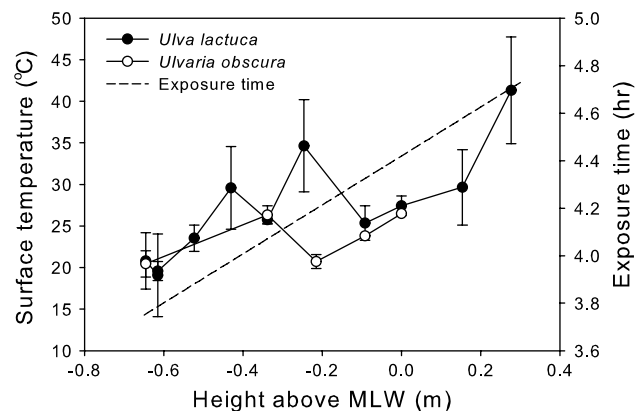
Fig. 5 Mean surface temperatures ( \pm 1 SD, N = 1 –9) of U. lactuca (black circles) and U. obscura (open circles) at different tidal heights immediately before they were immersed by an incoming tide. The dashed line indicates the amount of time that an alga would be exposed to the air during the low tide that occurred on the day that the measurements were taken based on estimates that were determined with Nobeltec Tides and Currents software
