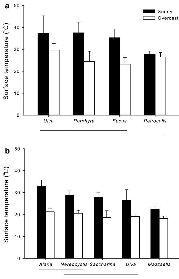
Fig. 4 Mean surface temperatures ( \pm 1 SD, N = 10 –15) of a the mid intertidal algae U. lactuca , Porphyra sp., F. distichus , and the “ Petrocelis ” stage of M. papillatus , and b the low intertidal algae A. marginata , N. luetkeana , S. latissima , U. lactuca and M. splendens on the Shannon Point Beach immediately before they were immersed by an incoming tide on a sunny (black bars) and an overcast day (white bars). Lines beneath the graphs indicate species for which means were not significantly different (Tukey’s test: P > 0.05 )
