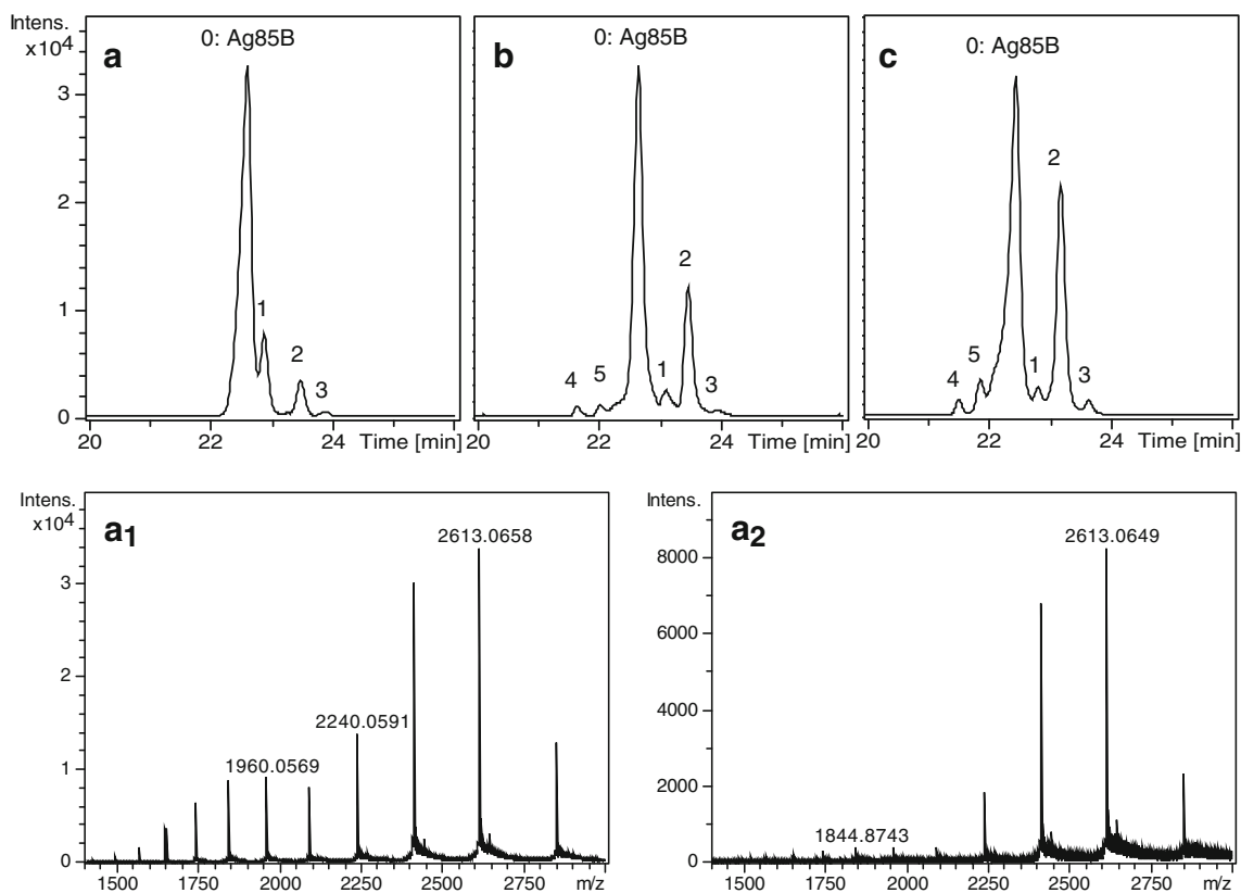
Fig. 2 BPEs obtained during CE-MS of Ag85B ( a ) and Ag85B which has been exposed to glycosylation conditions for 24 h at 25 °C ( b ) or at 37 °C ( c ). Mass spectra obtained at the apex of peaks 0 ( a 1 ) and 1 ( a 2 ) of BPE of Ag85B ( a )
