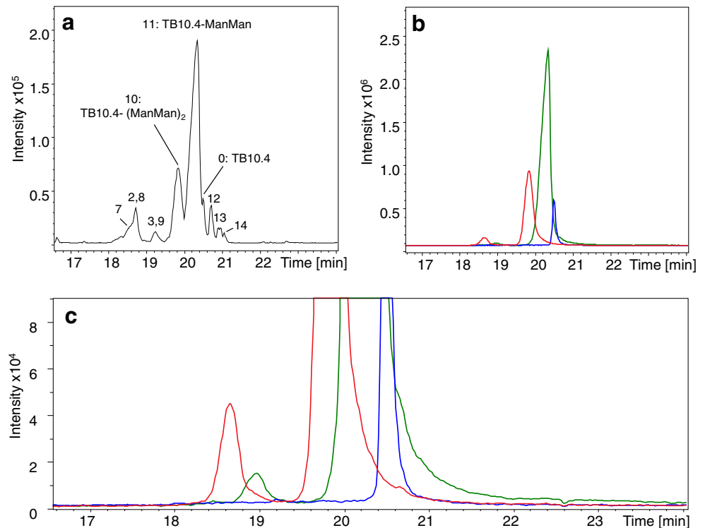
Fig. 3 BPE (a) and EIEs (b) of most abundant ions of TB10.4 (blue), monoglycosylated TB10.4 (green) and diglycosylated TB10.4 (red) obtained during CE-MS of TB10.4 conjugated with Man(1–6)Man. c zoom of b
