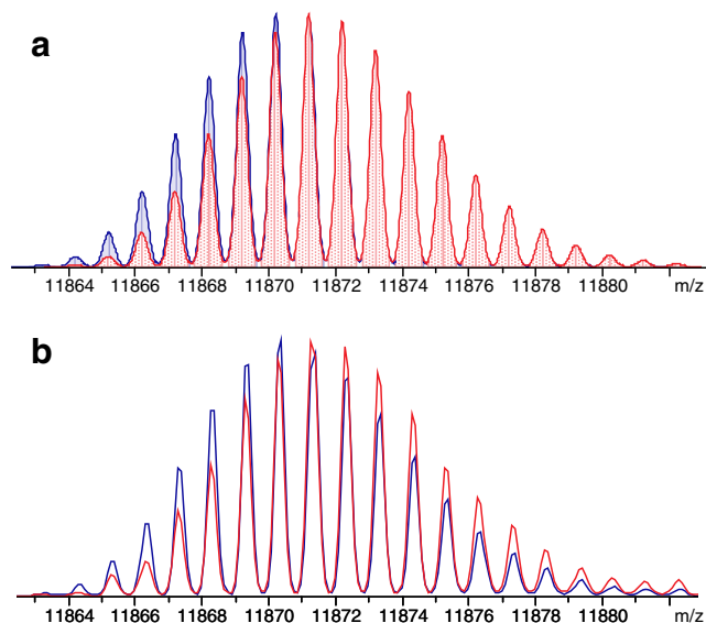
Fig. 4 Deconvoluted mass spectra showing isotopic pattern of TB10.4-[Man(1–6)Man] 2 (blue) and deamidated TB10.4-[Man(1–6)Man] 2 (red) obtained a in silico and b during CE-MS
