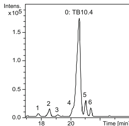
Fig. 1 BPE obtained during CE-MS of TB10.4 which has been exposed to glycosylation conditions at 37 °C for 24 h
