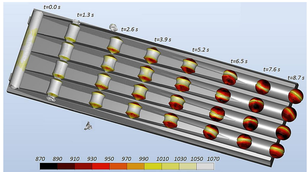
Fig. 8 Changes in workpiece shape in the cross-wedge rolling process for producing 70 mm diameter balls from a 51.5 mm diameter cylindrical rod
