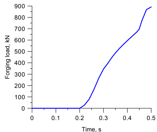
Fig. 3 Forging load during the side pressing of a rail head in a hexagonal pass
