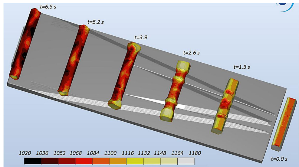
Fig. 5 CWR process for producing a cylindrical shaft and the distribution of temperature (in °C)
