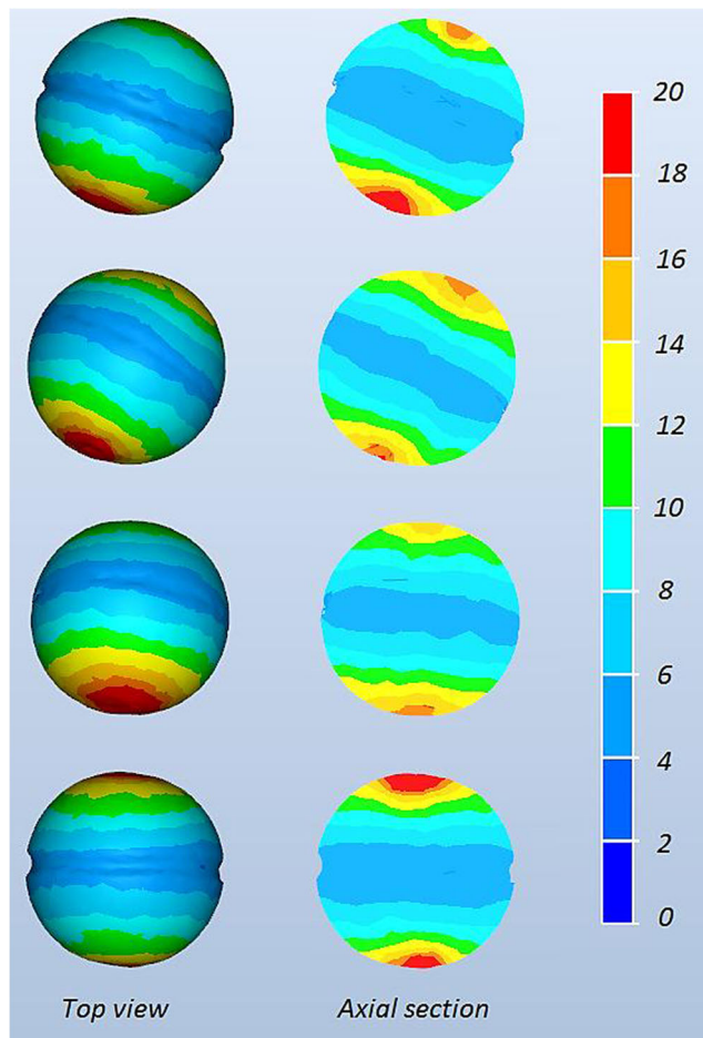
Fig. 9 Effective strain distributions in 70 mm diameter balls produced from scrap rail heads
