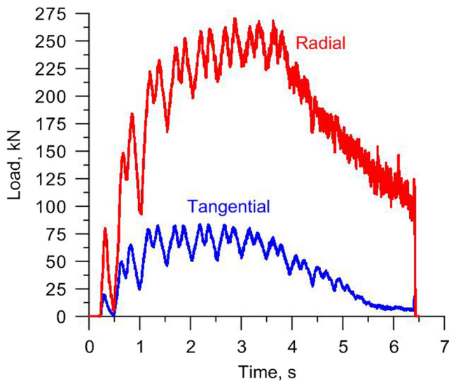
Fig. 6 Variations in the rolling force components during the forming of a 51.5 mm diameter cylindrical rod
