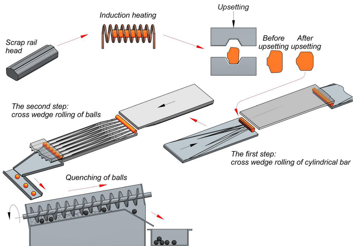
Fig. 1 Schematic design of an innovative process for producing balls from scrap rail heads
