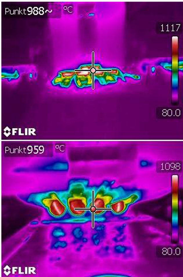
Fig. 13 Temperature measurement in the analyzed CWR process. Cylindrical shaft (top) and produced balls (down)
