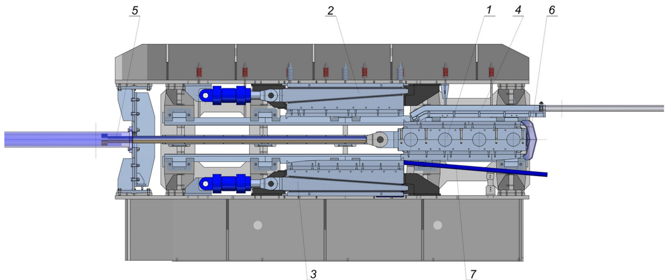
Fig. 11 Schematic design of the flat-wedge reversing mill designed at the Lublin University of Technology (description in the text)
