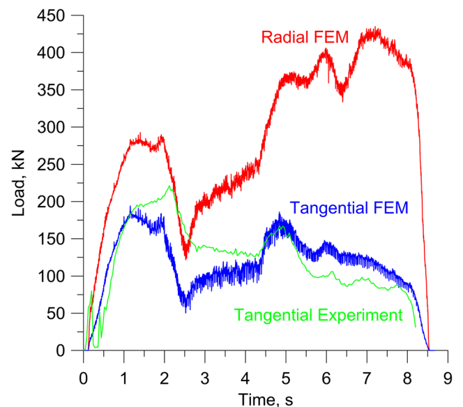
Fig. 10 Variations in the rolling force components during the forming of 70-mm diameter balls from 51.5 mm diameter rod
