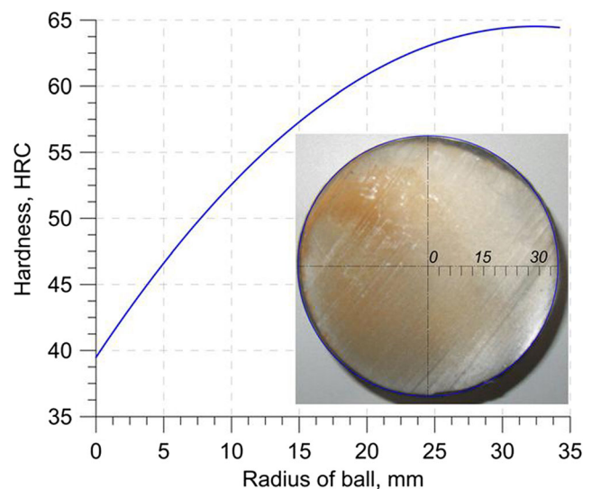
Fig. 15 Distribution of hardness in a ball produced by the proposed method
