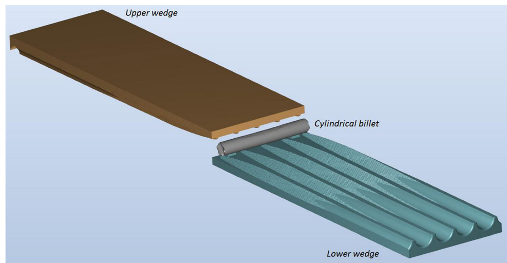
Fig. 7 Geometrical model of a cross-wedge rolling process for producing four 70 mm diameter balls from a 51.5 mm diameter cylindrical rod
