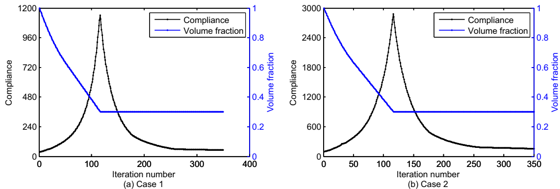
Fig. 11 Iterative histories of the objective function and volume fraction for case 1 in a and case 2 in b
