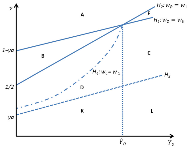
Fig. 1 Brunhilde’s strategy for a given Y_O
