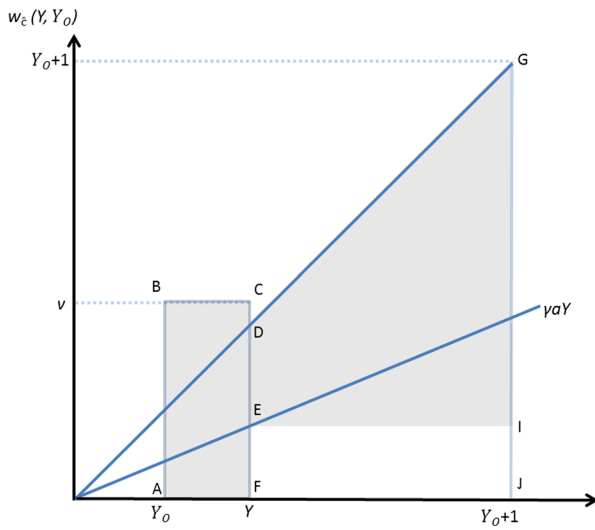
Fig. 2 Brunhilde's payoff for a given v and Y_0
