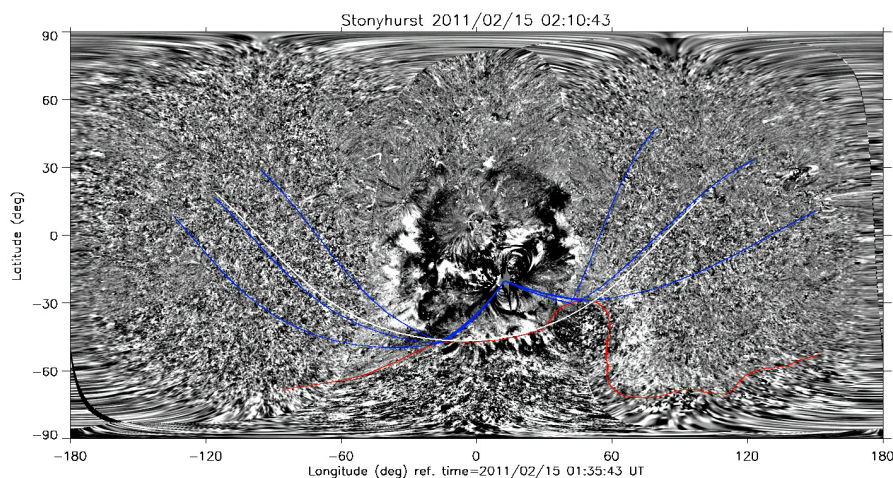
Figure 31: Still from a movie – An animation of the 2011 Feb 15 coronal wave and its reflection on a coronal hole as seen on a full sun map combining EUVI-A and EUVI-B (195 Å) with AIA (193 Å) data. Shown is a sequence of running ratio images. The blue lines indicate the predicted wave trajectories and clearly show the reflection at the coronal hole boundary (red line). Reproduced with permission from Olmedo et al. (2012), copyright by AAS. (To watch the movie, please go to the online version of this review article at http://www.livingreviews.org/lrsp-2015-3 .)
