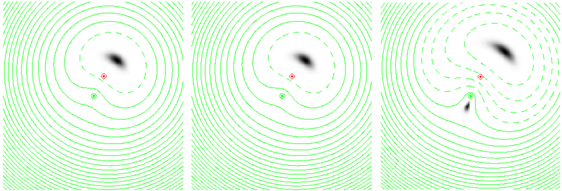
Figure 3: Illustration of a Fermat surface for a source (red symbol) close to the line of sight to a galaxy (green symbol). In each case the appearance of the images to the observer is shown by a greyscale, and the contours of the Fermat surface are given by green contours. Note that images form at stationary points of the surface defined by the contours. In the three panels, the mass of the galaxy, and thus the distortion of the Fermat surface, increases, resulting in an increasingly visible secondary image at the position of the saddle point. At the same time, the primary image moves further from the line of sight to the source. In each case the third image, at the position of the Fermat maximum, is too faint to see.
