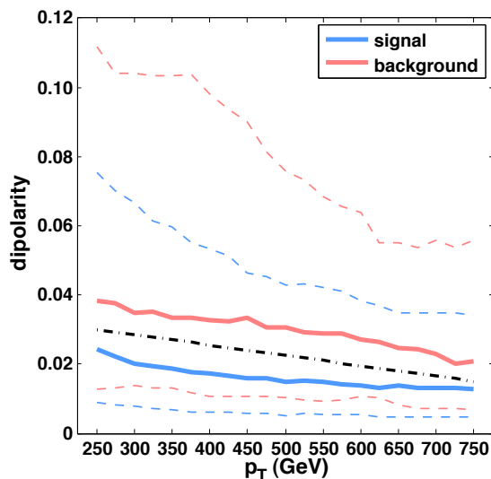
Figure 4. Dipolarity distributions for W^\pm s reconstructed by the HEPTopTagger and passing default mass cuts with m_{\text{filt}} \in [150 \text{ GeV}, 210 \text{ GeV}] . Thick solid lines indicate central values, whereas thin dashed lines correspond to values at 10% and 90%. Here and throughout the p_T is that of the fat R = 1.5 jet. For all p_T the central value of the dipolarity for the background is \mathcal{O}(50\% - 100\%) larger than for the signal. This figure uses the HERWIG event samples; the PYTHIA event samples yield similar distributions. The dot-dash line roughly indicates where dipolarity cuts are made at the S=20% working point.
