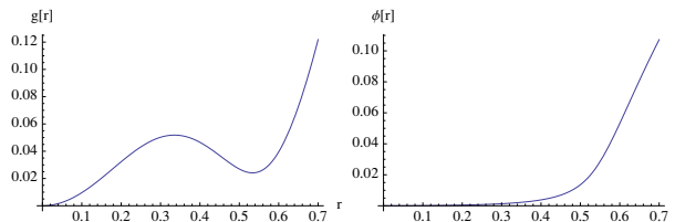
Figure 2. This plot of the emblackening factor g (left) and the electrostatic potential \phi (right) in the q_\varphi = 1.3, m_\varphi^2 = 0 groundstate solution exhibits the almost-RN horizon at r = 1 . In this plot and those below, we use units where \mu = 2\sqrt{3} .
