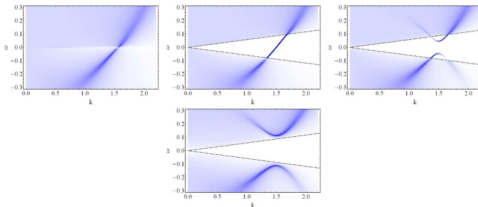
Figure 4. Mixing between positive- and negative-frequency modes due to the Majorana coupling. Shown are density plots of the fermion spectral density A(k, \omega) = \text{Im}G_{\mathcal{O}_2\mathcal{O}_2^\dagger} for q_\zeta = \frac{3}{4}, m_\zeta = 0 . The first plot is in the T = 0 RN black hole, no scalar. The remaining plots are in the zero temperature background with q_\varphi = \frac{3}{2}, m_\varphi^2 = 0 , for various values of the Majorana coupling, \eta_5 = 0, 0.2, 1.5 .
