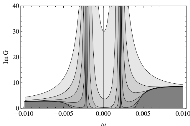
Figure 7. The effect of temperature (much less than T_c ) on the fermion spectral function. Shown are plots at q_\varphi = 1, m_\varphi^2 = -1, q_\zeta = \frac{1}{2}, m_\zeta = 0, \eta_5 = .025 , and momenta where the peak is closest to \omega = 0 . The different curves correspond to different temperatures approaching T = 0 .
