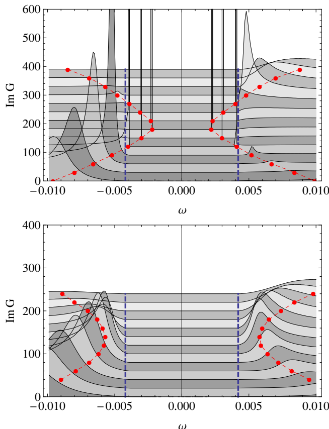
Figure 5. The effect of the Majorana coupling on the fermion spectral density. Shown are plots of A(k, \omega) at various k \in [.81, .93] for q_\zeta = \frac{1}{2}, m_\zeta = 0 in a low-temperature background of a scalar with q_\varphi = 1, m_\varphi^2 = -1 , with \eta_5 = 0.025 (top) and \eta_5 = 0.075 (bottom). The blue dashed line indicates the boundary of the region in which the incoherent part of the spectral density is completely suppressed, and the lifetime of the quasiparticle is infinite. The red dotted line indicates the location of the peak.
