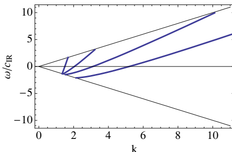
Figure 3. Boundstates outside the IR lightcone for various values of q_\varphi = 1.5, 2, 3, 5 . Note that the frequency axis has been scaled by c_{\text{IR}} which is different for each curve. We can't resist mentioning the approximate relation k_F \approx q_\varphi for where the curves cross \omega = 0 .
