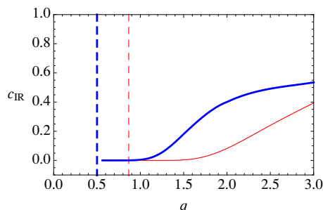
Figure 1. The speed of light in the IR CFT, c_{\text{IR}} , as a function of the boson charge. The blue thick curve is m_\phi^2 = -1 , the red thin curve is m_\phi^2 = 0 . The vertical dashed lines indicate the value of q_\phi below which the RN solution is stable.
