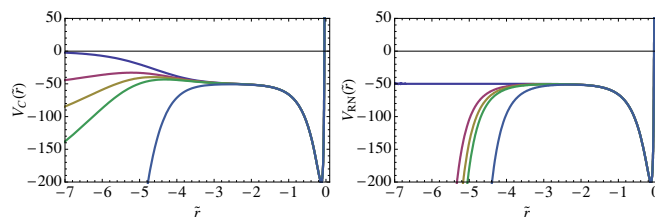
Figure 6. The effective Schrödinger potentials for a probe scalar with mass m_{\text{probe}}^2 = -3/2 and q_{\text{probe}} = 5 . The horizontal axis is the tortoise coordinate; the UV boundary is to the right, at \tilde{r} = 0 . The different curves are different values of \omega > 0 ; the top curve in each plot is for \omega = 0 . Left: The potentials for the groundstate with m_\varphi^2 = 0 and q_\varphi = 1 . Right: The corresponding pictures for the RN black hole with the same charge density.
