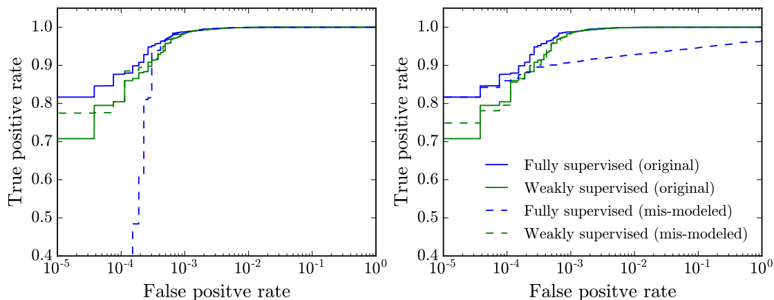
Figure 10. ROC curves showing the response of the network to mis-modeled data. The mis-modeling in the left panel shows the results of taking a random 15 % of the signal events and labeling them as background before training. The right panel demonstrates what happens under a phase space swap, where we mislabel the 10 % most signal-like background event and the 15 % most background-like signal events. The fully supervised network trained on the mislabeled data performs much worse at small false positive rates than when the data is not mislabeled. The weakly supervised network does not rely on individual event labels, and therefore has essentially no change in performance.
