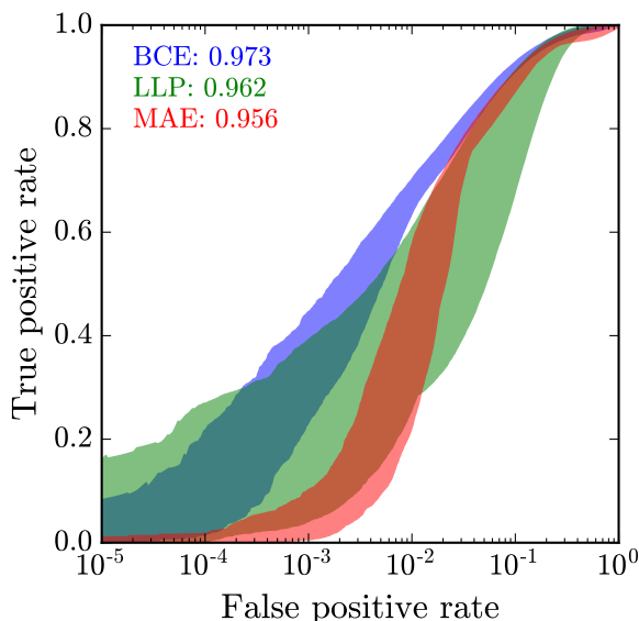
Figure 12. The spread in the ROC curves for 100 different trainings of weak supervision for different choices of the loss function. The mean area under the curve is denoted in the legend. The ordering of the legened matches the curves at a false positive rate of 10 -3 .
