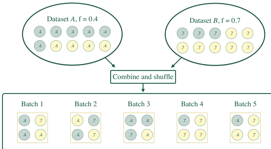
Figure 2. Schematic of the data flow. We are given (at least) two data sets and told to learn two different classes (yellow and green), without knowing the truth value of any one event. Instead, each event is only labeled with the ratio of yellows to the total that are in its dataset. The datasets are combined and shuffled into batches, that are used for training. For illustration in this figure, the batch size is four, and this represents one random permutation.
