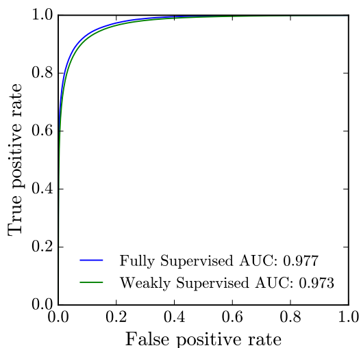
Figure 4. Receiver operator characteristic (ROC) curve for the weakly supervised and fully supervised networks. The performance is very similar for the two networks.
