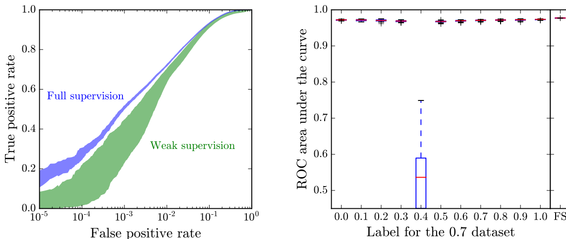
Figure 5. The left panel shows the spread derived from the 100 networks trained to compute the error bars. We show the result for both fully and weakly supervised networks; for the later, the network is trained using the correct choice of 0.4 and 0.7 for the labels. The area under the curve is very similar for all of them, but the curves differ in their variance and at very low values of the false positive rate, demonstrating the possible spread in network performance trained on the same data. The right panel shows a comparison of the fully supervised network (labeled “FS”) and the weakly supervised network when one of the datasets labels does not match its true ratio. One data set has a true ratio of 0.4 and is labeled as such. The other dataset has a ratio of 0.7, but the network is trained using the label as specified on the x -axis.
