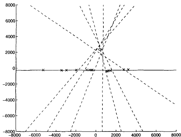
Fig. 5. The fixed points and lines obtained from all 7 possible sequential image pairs from sequence I (figure 3), with axes in pixels. \times are the epipoles, dashed and solid lines are the screw axes and the horizon respectively, o is the apex at (394, 2370) . The horizon line is at y = -255 .
