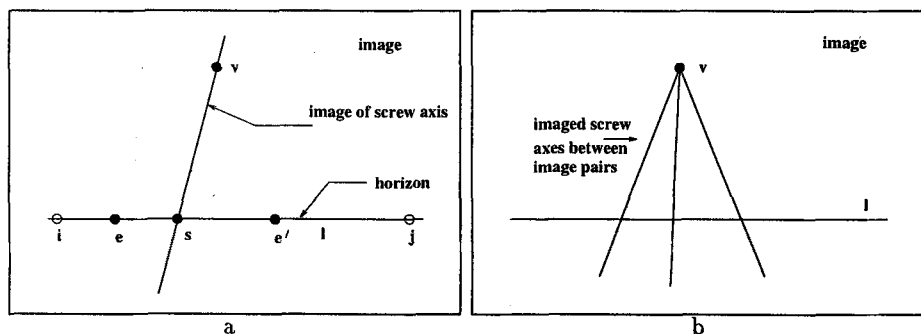
Fig. 2. Fixed image entities for planar motion. (a) For two views the imaged screw axis is a line of fixed points in the image under the motion. The horizon is a fixed line under the motion. (b) The relation between the fixed lines obtained pairwise for three images under planar motion. The image horizon lines for each pair are coincident, and the imaged screw axes for each pair intersect in the apex. All the epipoles lie on the horizon line.
