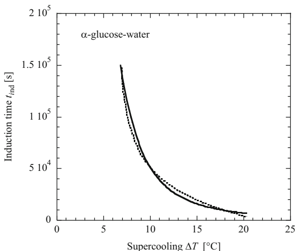
Fig. 7.1 Induction time as a function of supercooling. The solid line is the experimental value reported by Srisa-nga et al. [27], and the dotted line is a best fit of a theoretical equation. This graph was taken from Kubota [32]
