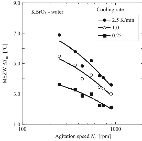
Fig. 7.2 The effect of agitation speed on MSZW for the potassium bromate-water system (Data were taken from Matsui and Harano [35])
