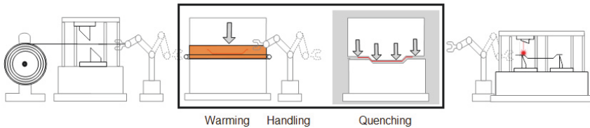
Fig. 1. Production line for the press hardening of sheet metal focusing on the three steps: (1) warming in a furnace unit, (2) handling with a robot system with grippers, and (3) quenching.
