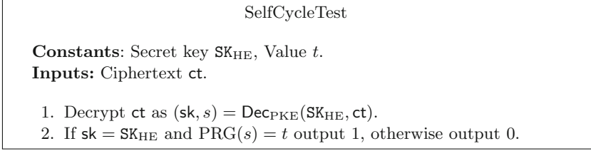
Fig. 3. SelfCycleTest
