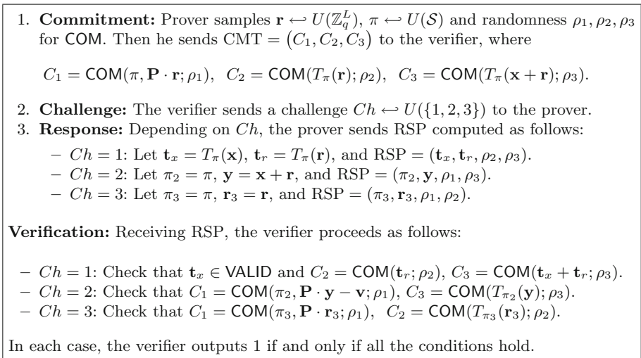
Fig. 1. A ZKAoK for the relation R_{\text{abstract}} .
