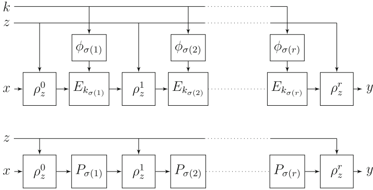
Fig. 1. The randomized key-length extension construction R[E] (top), and its induced sequential cipher \bar{R}[P] (bottom).
