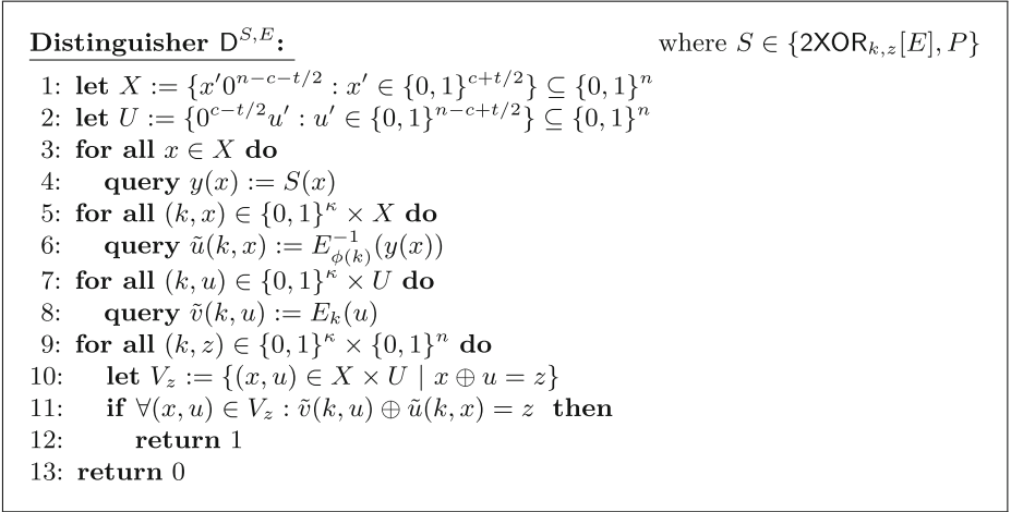
Fig. 3. Distinguisher D for the proof of Theorem 3, attacking the construction 2XOR and parametrized by c, t .
