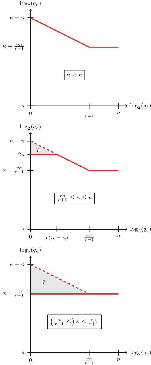
Fig. 7. The security of plain cascade encryption with 2r + 1 or 2r + 2 rounds, depending on \kappa and n . All parameters below the solid line are secure due to Theorem 6 or the results of [9]. All parameters above the dashed line are insecure due to the attack of [12]. The status for parameters between these lines remains unknown.
