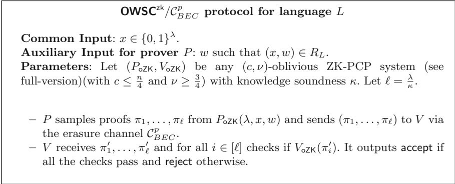
Fig. 3. Realizing zero-knowledge from binary erasure channel
