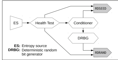
Fig. 1. Overview of the ISK-RNG
