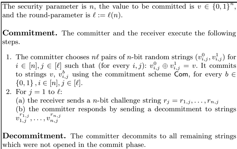
Fig. 1. The PRS Preamble based on \text{Com}
