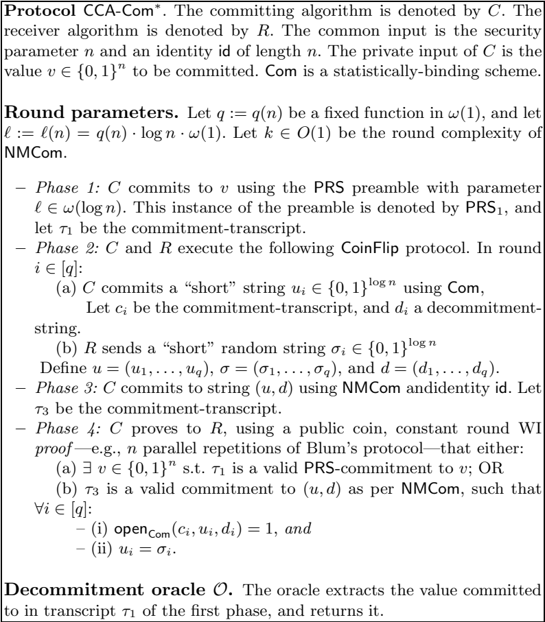
Fig. 4. Protocol CCA-Com* based on one-way functions
