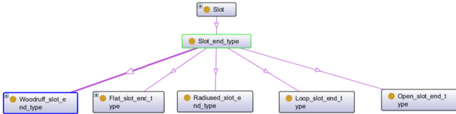
Fig. 2. OntoSTEP-NC graph
