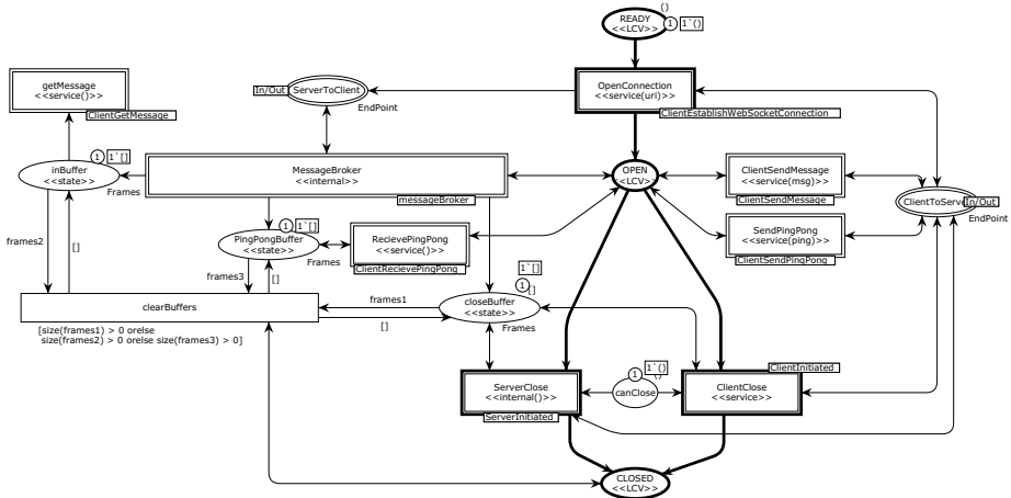
Fig. 2. The Client principal module
