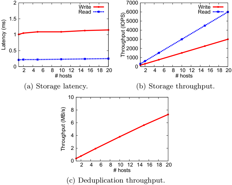
Fig. 3. DEDIS results for up to 20 cluster nodes with mixed storage writes and reads
