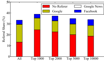
Fig. 5. Referral shares for interesting-URLs
