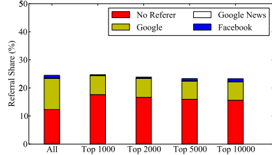
Fig. 4. Referral shares for user-URLs
