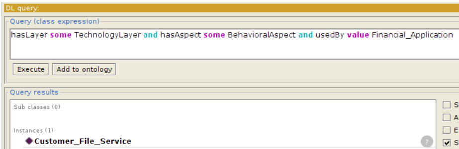
Fig. 2. Query Result
