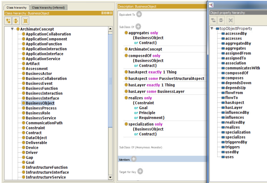
Fig. 1. Business Function class and corresponding properties
