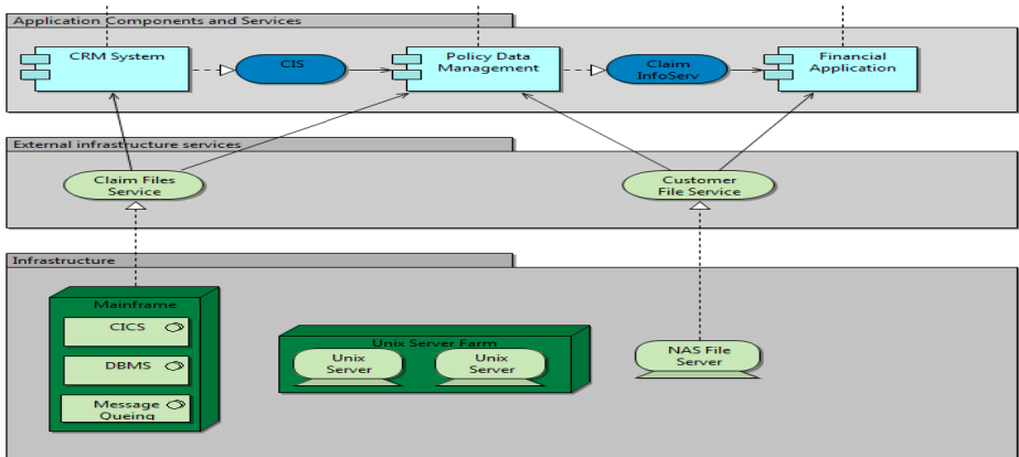
Fig. 3. ArchiSurance Layered View
