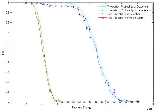
Fig. 8. Theoretical and Real Probabilities ( T_S^{SU} = 0.0512s )
