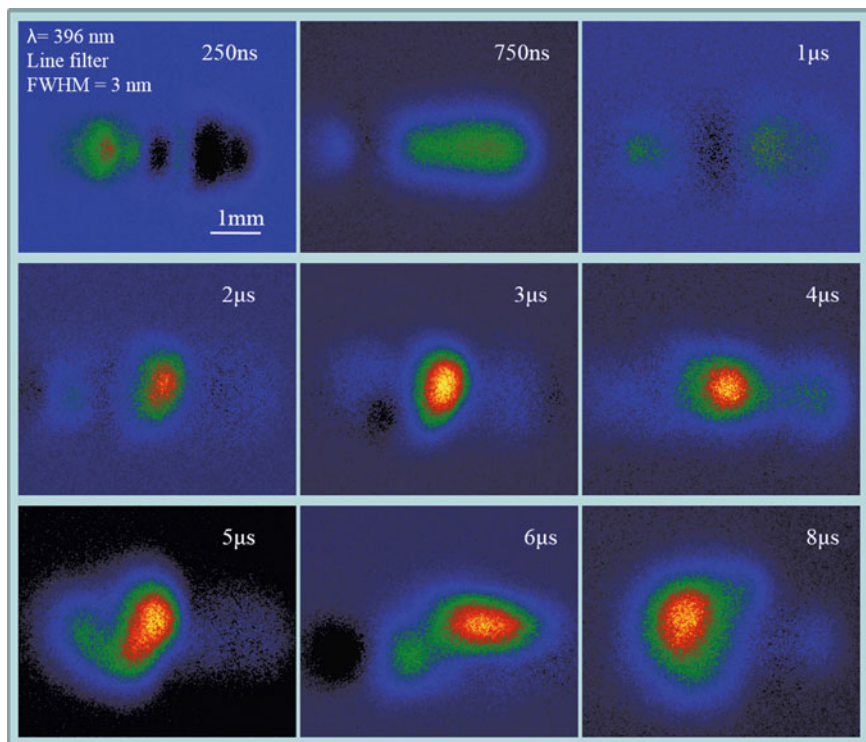
Fig. 9.15 Spectral images of Calcium diffusion measured temporally. Calcium line filter (396 nm) was used with line width of 3 nm. The bar represents 1 mm. (figure reprinted from P. K. Diwakar, S. Groh, K. Niemax, D. W. Hahn, J. Anal. At. Spectrom. , 2010, 25, 1921–1930—Reproduced by permission of The Royal Society of Chemistry)
