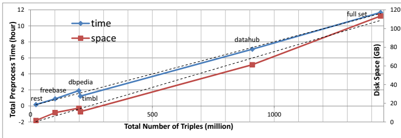
Fig. 5. Preprocessing: Time/Space - Total Triples
