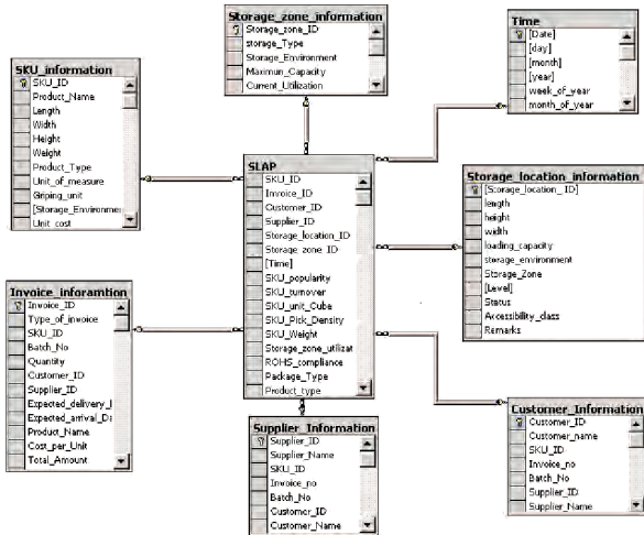
Fig. 2. The relational database structure of DCAM
