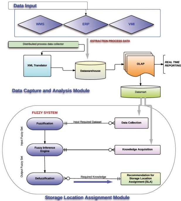
Fig. 1. Fuzzy Storage Assignment System Algorithm
