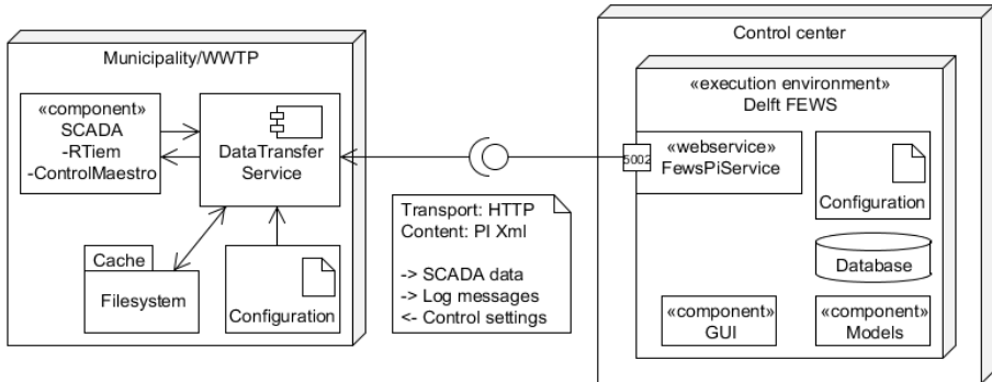
Fig. 3. Schematic representation of webservice hosted by Delft-FEWS
