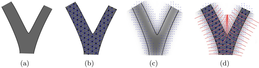
Fig. 1. Graph columns construction based on flow lines. Graph columns are generated from an initial coarse segmentation as shown in (a). This initial segmentation is converted to a surface mesh, where vertices of the graph columns are at the center of each surface voxel face as depicted in (b) by black dots. Subsequently, the coarse initial segmentation is smoothed and a gradient vector field is computed, see (c). Finally, (d) shows the graph columns represented by red lines which trace this gradient field from the vertices located at the mesh surface.
