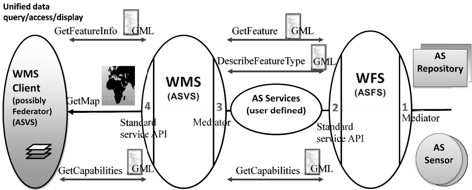
Fig. 3. Application of ASIS to GIS Domain
