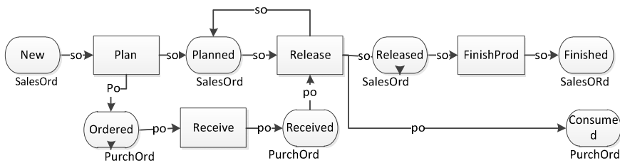
Fig. 1. Petri Net for Assemble to Order process
