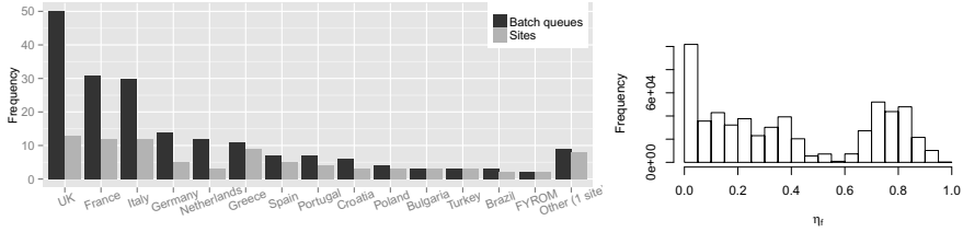
Fig. 1. Distribution of sites and batch queues per country in the biomed VO (January 2013) ( left ) and histogram of fineness incident degree sampled in bins of 0.05 ( right )
